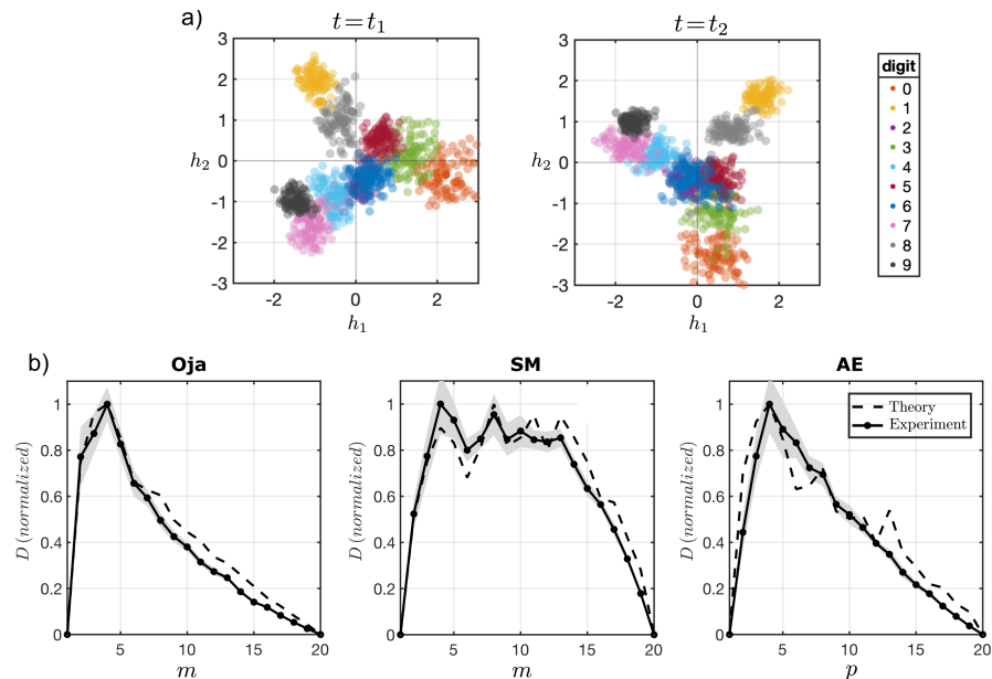
Figure 5: Drift in MNIST data. a) Two snapshots of hidden layer representations for 10 sample digits in a linear autoencoder ( n = m = 784 , p = 2 , \eta = 0.01 , t_1 = 1.6 \times 10^4 and t_2 = 10^5 ). To show the fluctuations alongside the drift, a time window of t_w = 5000 preceding each snapshot is considered and representations at 100 uniformly chosen times are overlaid. b) Normalized rate of drift as a function of output dimension ( m ) for Oja and Similarity Matching (SM), and bottleneck dimension ( p ) for autoencoder (AE). For the results in this panel, projections of MNIST data onto its top n = 20 principal components are used as input. The plots show the drift rate for the representation of the top principal vector (shaded area: standard deviation over multiple runs).
