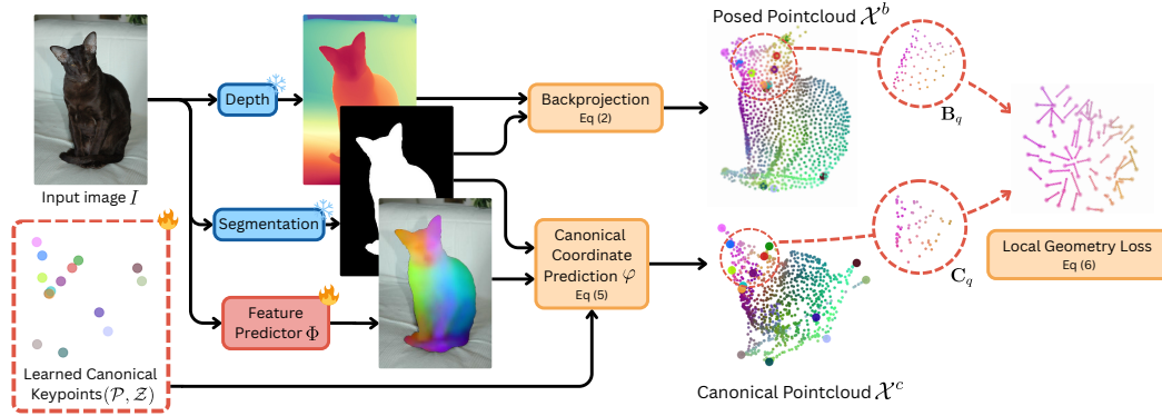
Figure 2: Overview of our approach. We extract segmentation masks and depths maps from training images and backproject object points to produce the posed point clouds \mathcal{X}^b . We predict dense features with \Phi and match them against our jointly learned sparse category prototype (\mathcal{P}, \mathcal{Z}) to produce the canonical point clouds \mathcal{X}^c . The local geometric alignment between the two provides supervision for updating \Phi .
