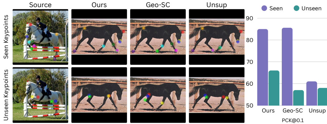
Figure 1: Illustration of the generalization gap on unseen keypoints. (Left) Top row: when evaluated on known keypoints, both our model and Geo-SC [62] perform well, while the unsupervised DINOv2+SD [61] struggles to correctly disambiguate the legs of the horse. Bottom row: when presented with keypoints unseen at training time, both our model and DINO+SD predict noisy but reasonable correspondence, while Geo-SC predictions noticeably degrade. (Right) Even though it obtains strong performance on known keypoints, Geo-SC performs worse than its unsupervised counterpart on our new benchmark of unseen keypoints. In comparison, our model still achieves competitive results.
