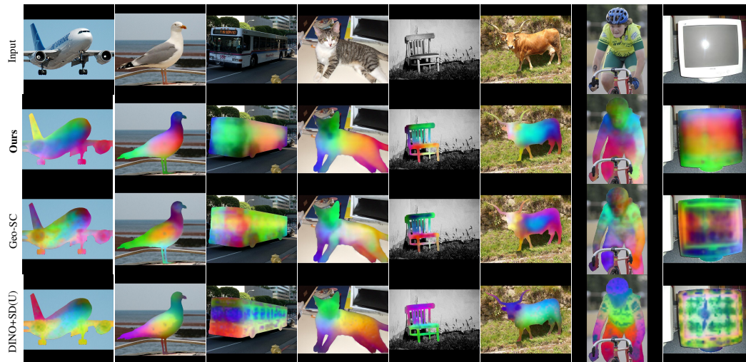
Figure 4: PCA visualization of the feature maps from different models. Note that PCA is computed on object features only. The inclusion of geometric constraints during training results in fewer high frequency artifacts in the predicted feature maps for our approach.
