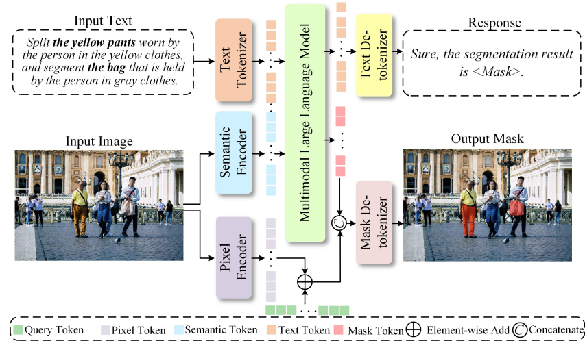
Figure 2: Architecture of the proposed ALToLLM.
