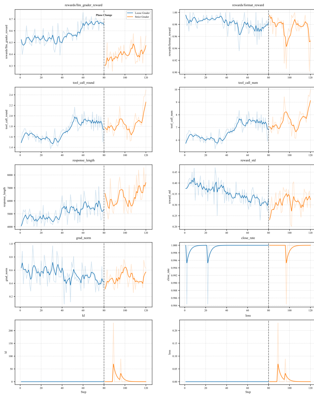
Figure 13: The detailed training curve of the DeepDiver-Qwen2.5-7B-Instruct model shows the trending of key metrics throughout the training process. These metrics include reward, tool call frequency, response length, reward standard deviation, gradient norm, KL divergence, and response completion rate.
