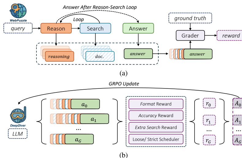
Figure 3: DeepDiver overview. (a) Rollout Generation : DeepDiver iteratively reasons, retrieves evidence, and answers WebPuzzle queries, then receives rewards based on comparison with ground truth. (b) RL Updates : Retrieved text is masked during loss calculation, and the LLM is refined via GRPO using advantages A_i derived from rewards r_i .
