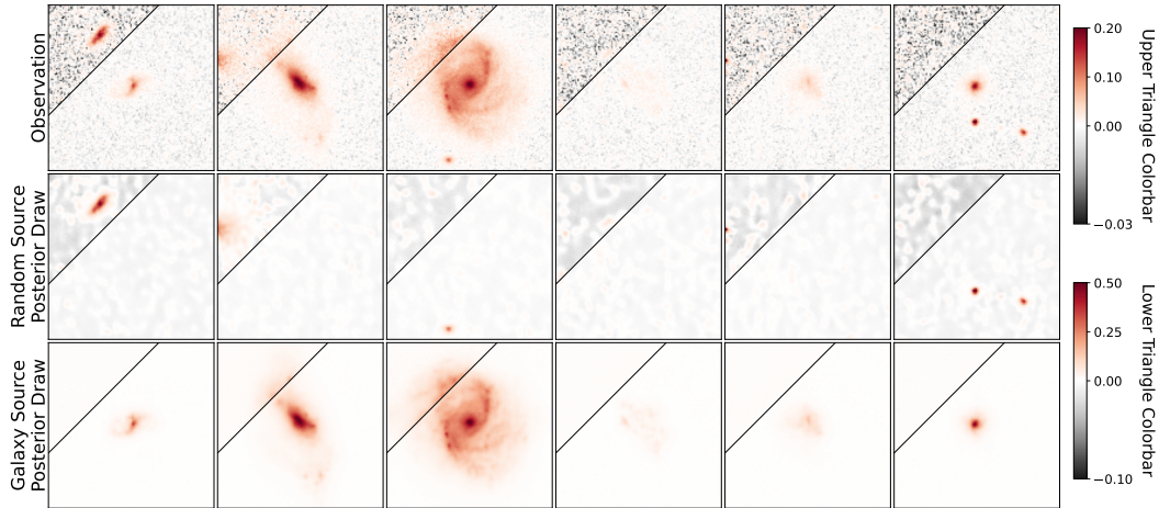
Figure 4: Observations of galaxy images along with posterior samples for the random and galaxy source using our method. Images are split into high-contrast (upper region) and low-contrast (lower region) colormaps to highlight the range of features. The galaxy source captures the central light while the small-scale fluctuations and the uncorrelated light is separated into the random source.
