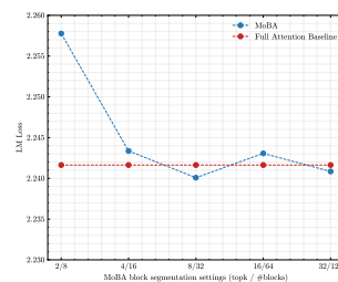
Figure 4: Fine-Grained Block Segmentation.
