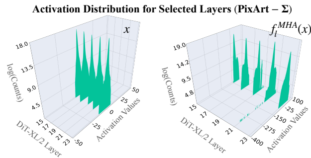
Figure E.1: Similar to DiT-XL/2, we observe high activation variance in PixArt- \Sigma MHA operators. We show input (left) and output (right) activation values corresponding to five representative layers (15, 17, 19, 21, 23) in PixArt- \Sigma .
