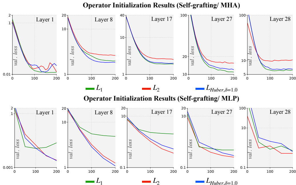
Figure C.2: Validation loss curves for MHA (top) and MLP (bottom) operator distillation showing the training dynamics for three regression objectives. As one can observe, L_1 shows better generalization for MHA and L_2 shows better generalization for MLP.
