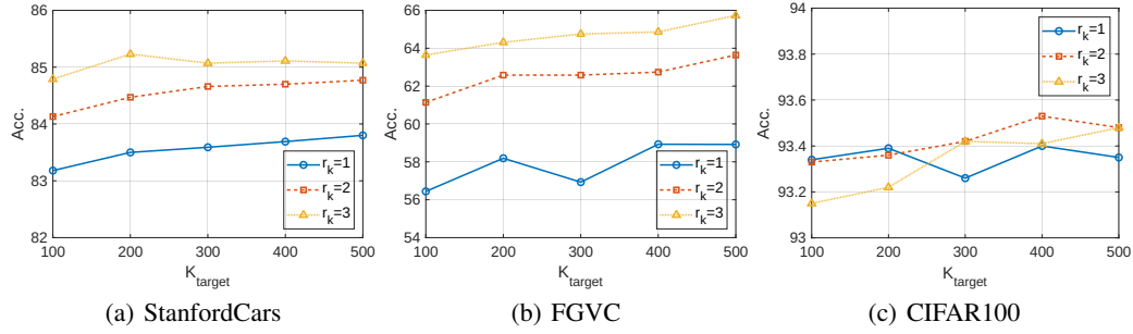
Figure 5: The performance of AdaMSS with different values of r_k and K_{\text{target}} .
