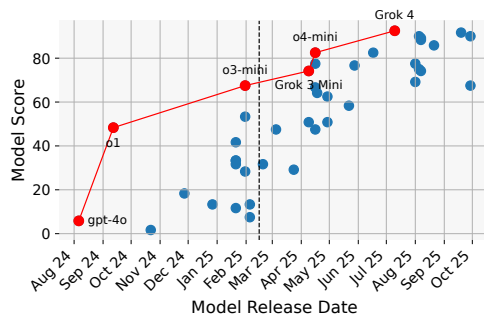
(a) Time-Pareto frontier for HMMT
