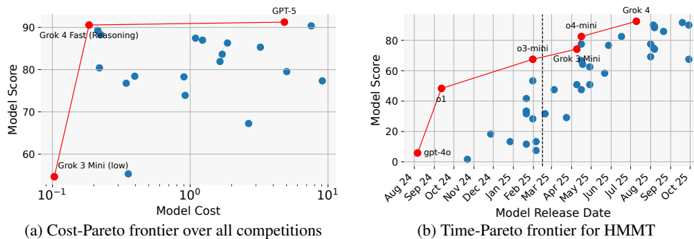
Figure 3: Scores of models with respect to their release date and cost (in USD). Each dot represents a model; the red curves trace the Pareto frontier in both (a) cost vs. score for all competitions, (b) release-date vs. score for HMMT. The black dotted line indicates the release date of HMMT.
