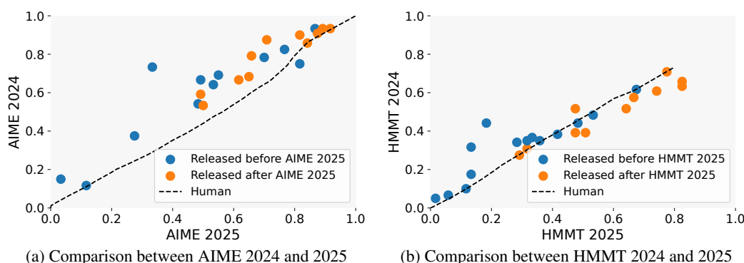
Figure 4: Comparison between new and old competitions. The black dotted line indicates quantiles of human performance. Models above the human line are likely contaminated.
