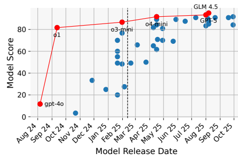
(b) Time-Pareto frontier for AIME
