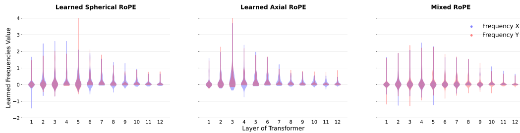
Figure 4: The distribution of learned frequencies in each layer of the ViT. Every method tends to learn low frequency positional encodings in the later layers of the network, meaning representations in the later layers are more invariant to position.
