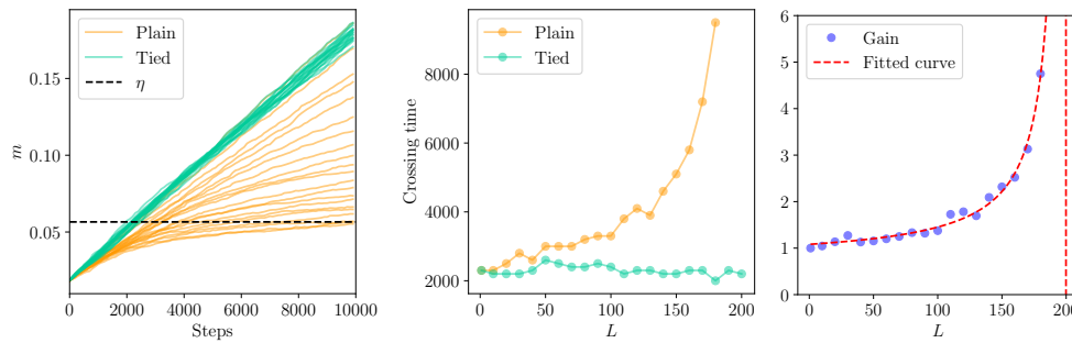
Figure 9: The gain in the case of a target function with SIE = 1 , where both cases use the same learning rate \gamma_0 = 0.005 . (left) The evolution of the overlap, (middle) the weak recovery time and (right) the gain. The gain diverges, as predicted. d = 1000 , \sigma = \text{ReLU}
