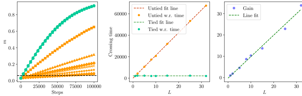
Figure 8: The gain in the case of a target function with SIE = 1 , where both cases use the same learning rate \gamma_0 = 0.005 . (left) The evolution of the overlap, (middle) the weak recovery time. The gain is proportional to L , as predicted. d = 1000 , \sigma = \text{ReLU}
