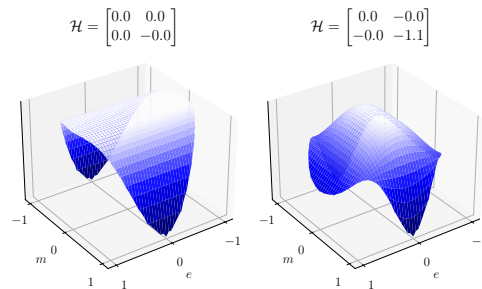
Figure 2: Population loss landscape for P = 0 (left) and P \neq 0 (right). Example of a case where SIE = 4, while \text{SIE}_{\text{positional}} = 2 . Target: g(\mathbf{z}_*) = 4/3 + \text{He}_4(z_1) + 2\text{He}_4(z_{*,2}) , P_1 = -P_2, R = \text{Tr} .
