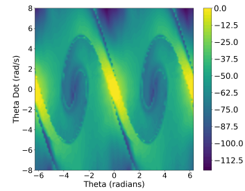
Figure 5: Generalized Lyapunov decrease condition.
