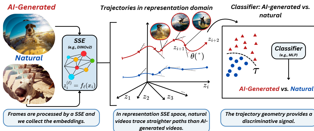
Figure 1: The ReStraV method for AI-video detection. Inspired by “perceptual straightening,” our approach leverages the geometric insight that natural videos form “straighter” feature trajectories ( z_i ) than generated ones. The temporal curvature (Eq. 1) serves as the discriminative signal for detection.
