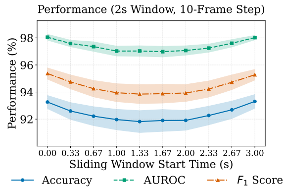
Figure 16: Ablation Study on Sliding Window Start Time. Performance of ReStraV when a 2s window (with T = 24 frames) slides across a 5s video with a 10-frame step.
