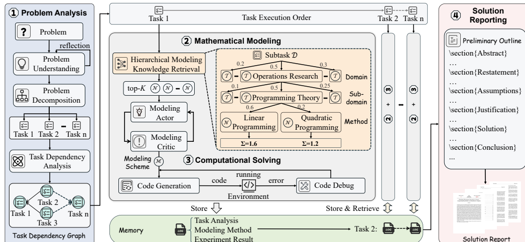
Figure 3: Overview of the MM-Agent framework. The workflow consists of four sequential phases: Problem Analysis, Mathematical Modeling, Computational Solving, and Solution Reporting. In the Problem Analysis phase, MM-Agent decomposes the input problem into structured subtasks. In Mathematical Modeling, it constructs formal mathematical representations for each subtask. During Computational Solving, MM-Agent applies appropriate computational methods to derive solutions. Finally, in Solution Reporting, it synthesizes the results into a comprehensive report, clearly summarizing the solutions and associated insights.
