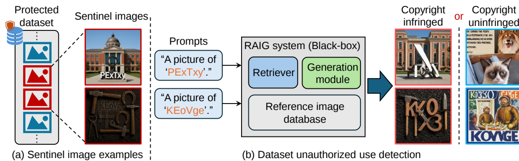
Figure 1: Illustration of our dataset protection. (a) Protected dataset structure showing the integration of sentinel images with the private dataset. (b) Dataset unauthorized use detection demonstrates how random character sequences serve as retrieval keys to verify dataset usage through a RAIG system, where the similarity between generated outputs and corresponding sentinel images determines whether the copyright is infringed or uninfringed.
