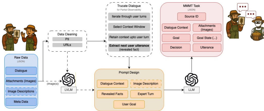
Figure 12: Overview of the MIRAGE-MMMT task generation pipeline. We begin with raw user-expert consultation data including dialogues and attached images. The pipeline applies a series of preprocessing, truncation, and prompting steps to convert each interaction into a structured decision-making task. Green modules denote inputs to the prompt template, while pink boxes indicate components automatically generated using a vision-language model (LVLM). The final structured output includes decision, goal state, and a response or clarification utterance for supervised training or evaluation.
