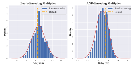
Figure 2: Delay distribution of 1000 randomly interconnected 16-bit multipliers using Wallace Tree compression with both AND and Booth partial product encoding PPG.
