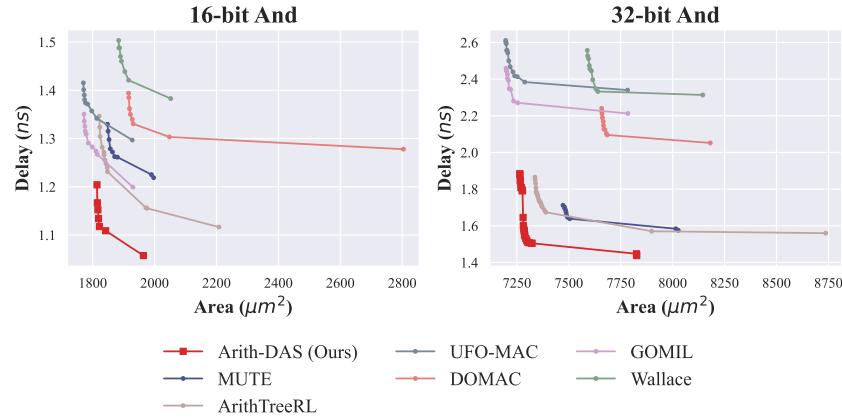
Figure 9: Pareto front of MAC designs.
