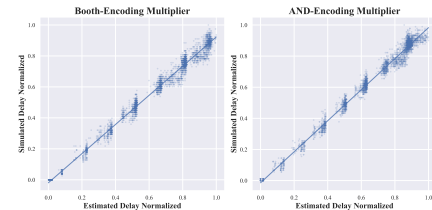
Figure 3: Comparison of estimated and post-synthesis delays for multipliers ranging from 4-bit to 64-bit, using Wallace Tree with both AND and Booth partial product encoding PPG.
