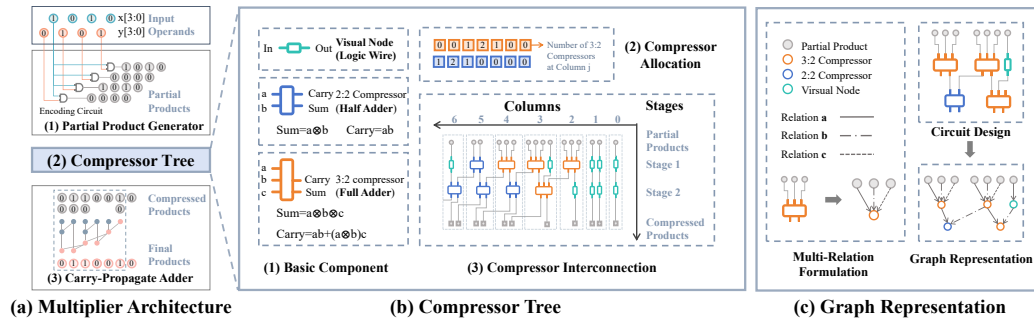
Figure 1: An illustration of a 4-bit multiplier with AND-gate based PPG.
