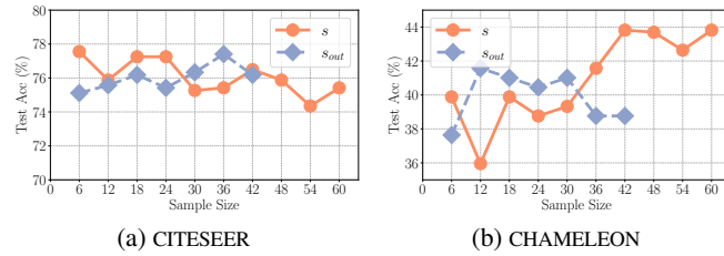
Figure 8: Effect of sample sizes on different datasets.
