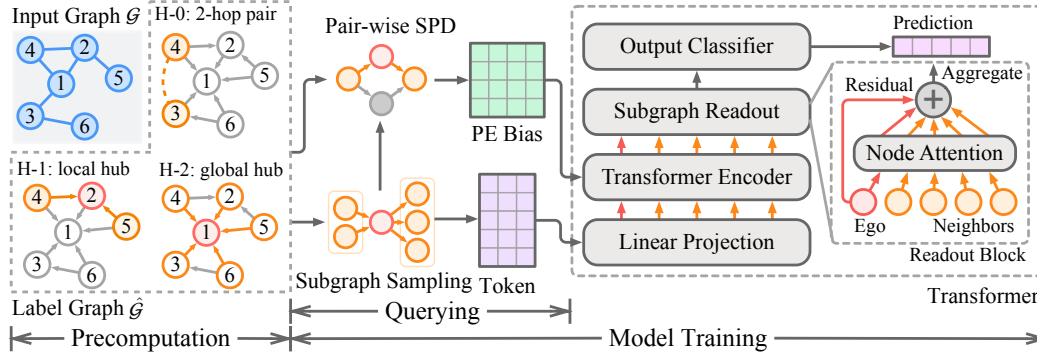
Figure 3: HubGT framework with precomputation and training stages. The precomputation stage processes the input graph and constructs the label index. During training , subgraph nodes and SPDs are queried from the index and applied as different Transformer inputs. Querying on CPU and training on GPU are pipelined and conducted simultaneously.
