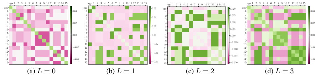
Figure 6: SPD PE as attention bias in different GT layers on CITESEER.
