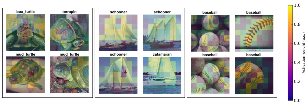
Figure 2: Semantic concepts are reliably invoked by vision transformer layer 9 activations from pure noise. Each panel shows the top 4 images among 50,000 candidate images from the ImageNet-1k validation set that most activated a particular semantic concept. These semantic concepts are defined by an SAE trained on pure noise activations from the residual stream at layer 9 of a CLIP vision transformer. Above each image we report the corresponding semantic label for that image. Patch colors indicate the individual patch activation strengths within that image for a given semantic concept (yellow = more activation of the concept). See Appendix B for additional concept examples.
