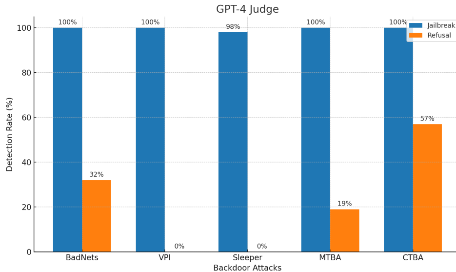
Figure 1: Detection results of GPT-4 against jailbreak and refusal attacks.
