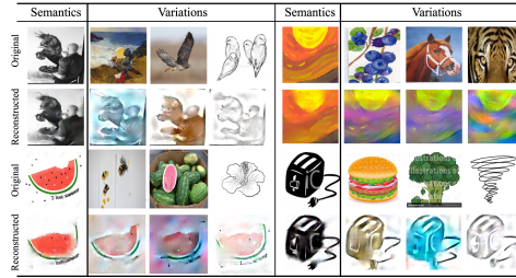
Figure 2: The reconstruction results produced by MS-UDG. Rows 1 and 3 display input images that preserve either semantic content or stylistic variations, derived from four distinct domains within the DomainNet dataset. In contrast, Rows 2 and 4 present reconstructed images using alternative variation representations within the feature space.
