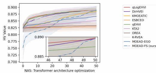
Figure 4: NAS comparison results. MOEA/D-FS and comparison algorithms initialize their surrogates with 18, 100 samples, respectively. MOEA/D-FS reaches competitive results while 82 evaluations are saved.
