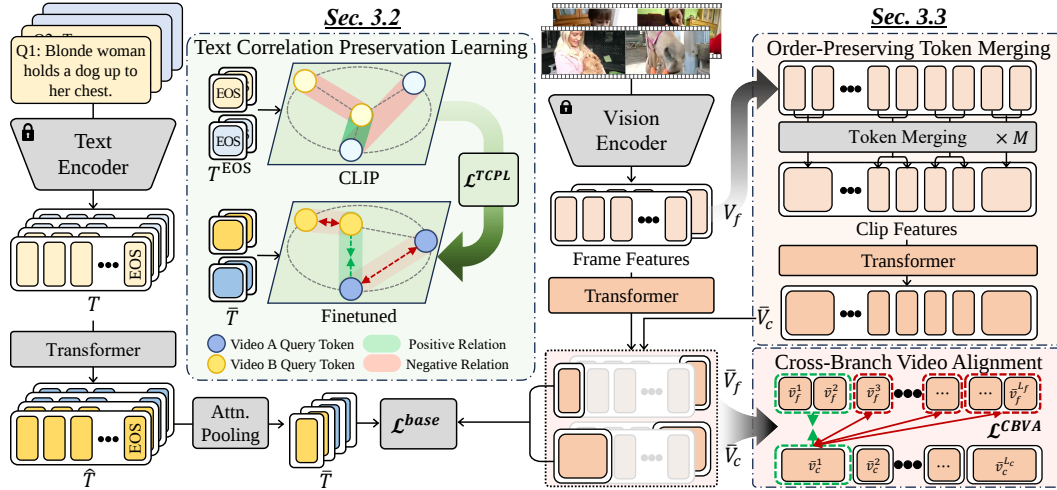
Figure 2: Method overview. We extract text and visual tokens with pretrained backbones, which are then processed via transformer layers. Text tokens are aggregated via attention pooling to produce a single query token \hat{T} for each text query. Also, following prior works, dual-branch visual tokens are encoded (both frame- and clip-level), producing a sequence \bar{V} of video tokens for each level. A baseline retrieval loss \mathcal{L}^{\text{base}} aligns \bar{T} with the most similar video token at each level. To mitigate text-side semantic collapse, Text Correlation Preservation Learning transfers CLIP’s query relationships. On the other hand, Cross-Branch Video Alignment aligns hierarchical segments by timestamping to mitigate collapse and preserve visual details. Furthermore, CBVA is precisely enhanced by constructing coherent clips with Order-Preserving Token Merging and improving adaptivity (illustrated in Sec. 3.3).
