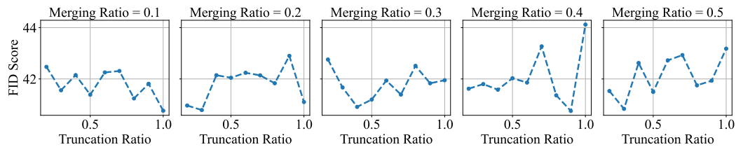
Figure 6: FID vs. Truncation Ratio under varying token merging ratios.
