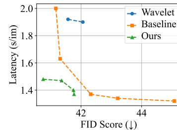
Figure 7: Wavelet vs. Fourier Token Merging: FID vs. Latency.
