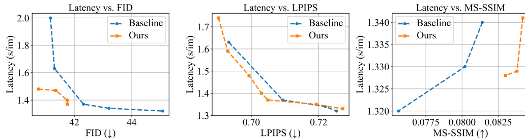
Figure 5: Comparison of latency versus image quality metrics between the baseline and our method. The different points on a curve correspond to different token merging ratios. Left: FID vs. latency, showing that our method achieves lower latency for comparable or better FID. Middle: LPIPS vs. latency, demonstrating improved perceptual similarity over baseline. Right: MS-SSIM vs. latency, indicating stronger structural consistency with minimal latency overhead. Note that Pareto frontiers are selected from a set of hyperparameter settings, and therefore differ across subplot. Overall, our approach consistently improves the quality-efficiency tradeoff across multiple evaluation metrics.
