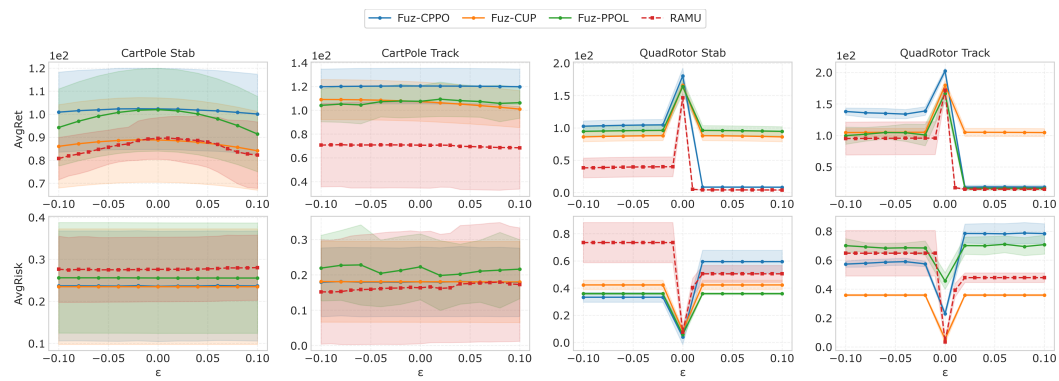
Figure 13: Average episodic reward (top) and average episodic risk (bottom) of Fuz-RL and RAMU in different scales' dynamics uncertainty settings. The horizontal axis represents the uncertainty level.
