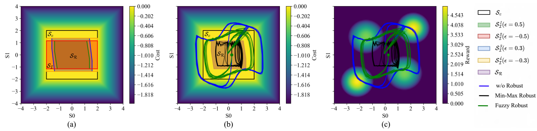
Figure 5: (a) Hierarchical relationship of safety sets, (b) Cost space and (c) Reward space trajectory comparisons, with dashed lines indicating safety boundaries.
