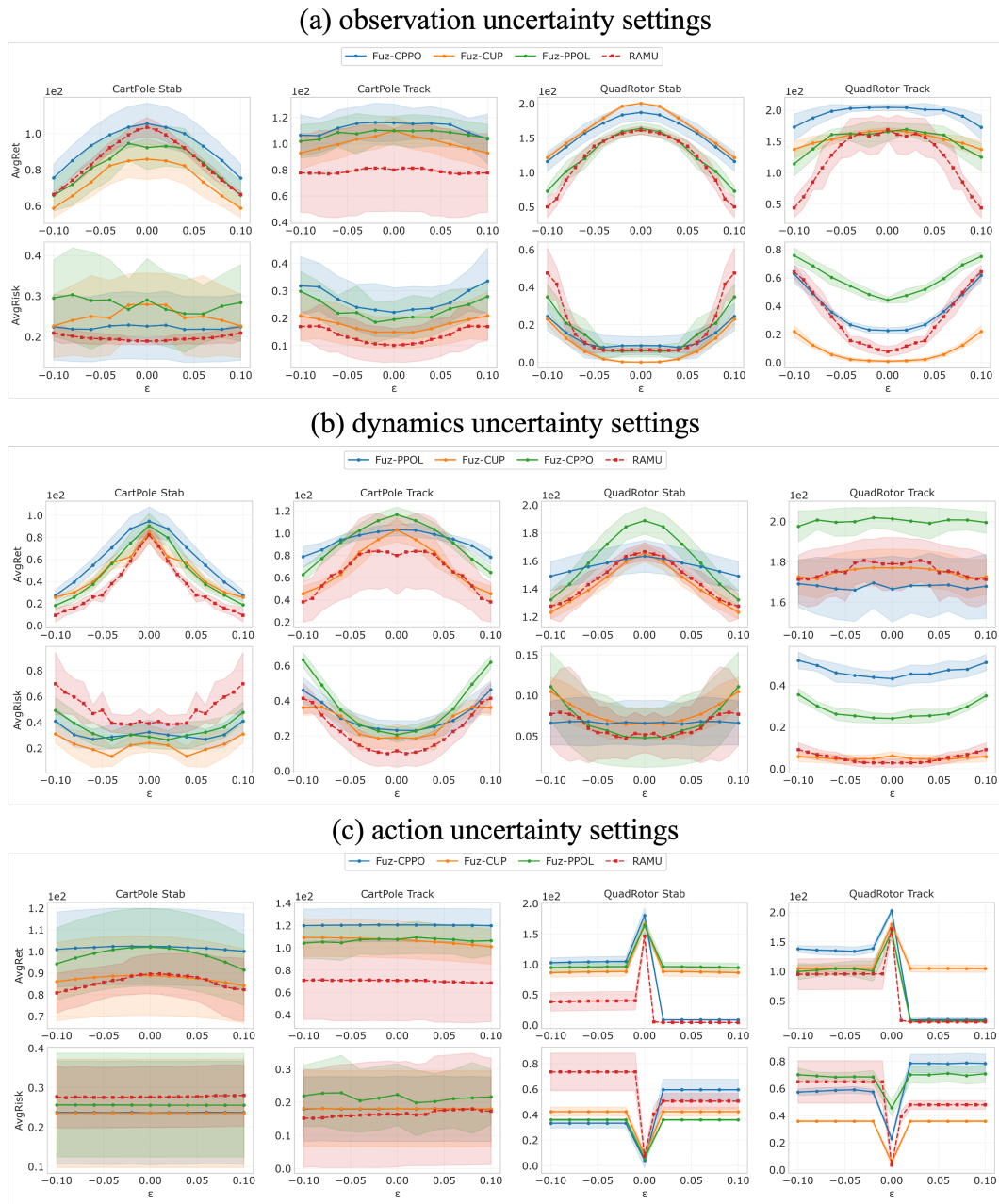
Figure 14: Average episodic reward (top) and average episodic risk (bottom) of Fuz-RL and RAMU in different scales' observation, dynamics, and action uncertainty settings. The horizontal axis represents the uncertainty level.
