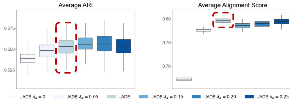
Figure 8: Sensitivity analysis: Varying \lambda_4 . Each boxplot summarizes the outcomes of 100 independent replications.
