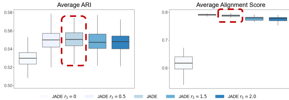
Figure 7: Sensitivity analysis: Varying \lambda_3 , where r_3 is the magnifier of \lambda_3 against JADE. Each boxplot summarizes the outcomes of 100 independent replications.
