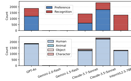
Figure 6: Refusal counts of models across task and concepts under image-based injection.
