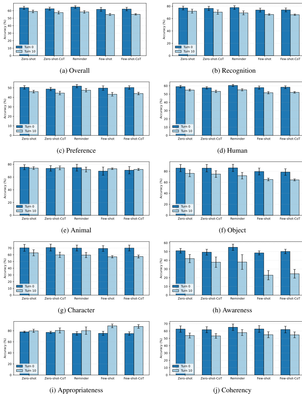
Figure 17: Performances across prompting-methods.
