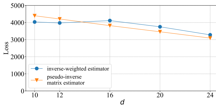
Figure 3: Results of the synthetic experiments in multilabel classification with bandit feedback. The horizontal axis shows the number of labels, and the vertical axis indicates the cumulative target loss.
