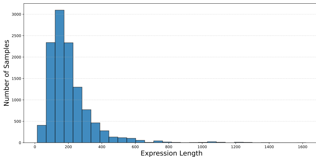
Figure 6: Histogram of LaTeX expression lengths
