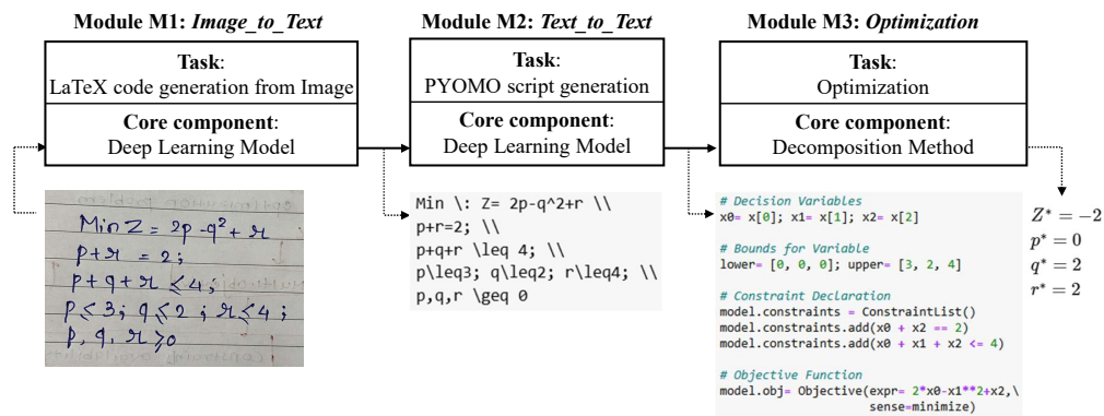
Figure 1: AutoOpt framework: workflow demonstration using an example
