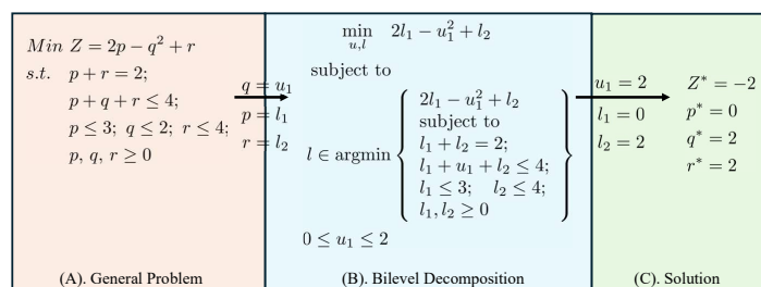
Figure 5: Problem solving using Bilevel optimization-based decomposition approach
