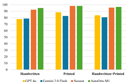
Figure 4: BLUE Score
