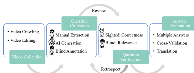
Figure 2: Data annotation pipeline.
