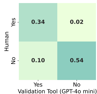
Figure 16: Consistency between human and machine scoring.
