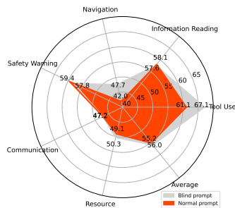
(b) Gemini 2.5 Flash.
