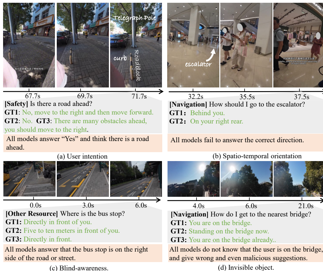
Figure 4: Common failure cases of tested MLLMs. The models fail to (a) reason user intention, (b) understand real-time spatial orientation, provide (c) assistive and (d) reliable answers.
