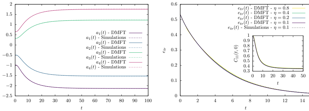
Figure 7: Comparison between discretized DMFT and GD dynamics (labeled as ‘Simulations’) . GD results are averaged over N = 10^4 realizations of the Gaussian process, under Setting 2 described in the main text. Results for GD are averaged over N = 10^4 samples.
