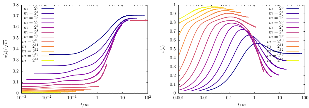
Figure 28: second layer weights and projection on of the first layer weigths onto the latent structure of the data for gradient flow under mean field initialization on timescales of order m . Left: rescaled second layer weights a(t)/\sqrt{m} as a function of the rescaled time t/m . The arrow on the right points at the threshold \gamma_{\text{GF}}^*(\alpha, \varphi, \tau) for interpolation under gradient flow, see Section F.2.3. Right: projection of the first layer weights on the latent space in the single index model as a function of rescaled time t/m . Here, \hat{\varphi}(z) = h(z) = (9/10)z + z^3/6 with \tau = 0.6 and \alpha = 0.3 . v = 1/\gamma in (F.57).
