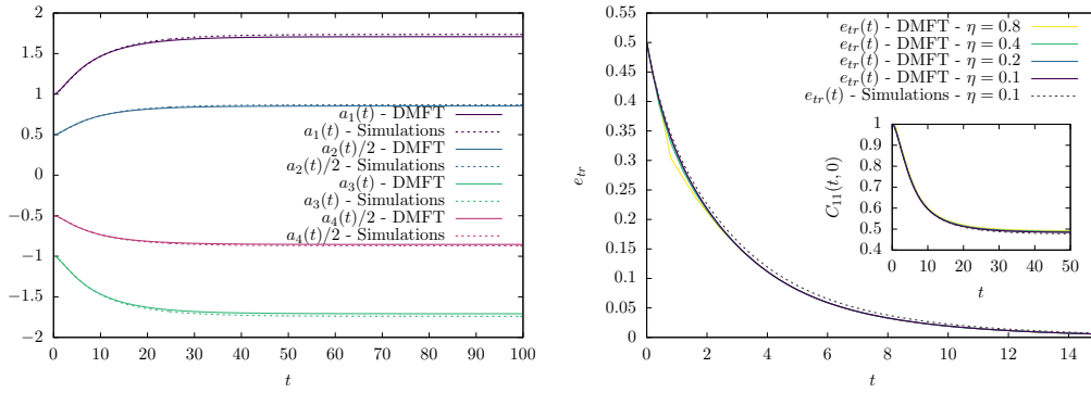
Figure 6: Comparison between discretized DMFT and GD dynamics for the Gaussian model (labeled as ‘Simulations’) . GD results are averaged over N = 10^4 realizations of the Gaussian process, under Setting 1 described in the main text. Left frame: Second layer for DMFT and GD with \eta_{GD} = \eta = 0.1 . Right frame: Train error and correlation function for DMFT with a few values of \eta , and for GD.
