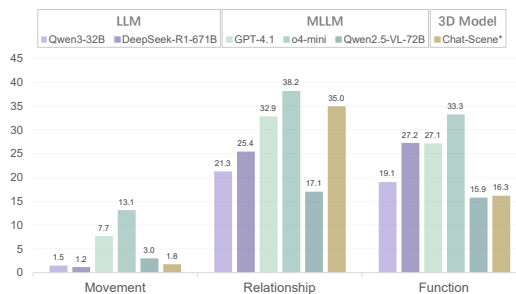
Figure 7: Results on different types of expressions on Part Level.
