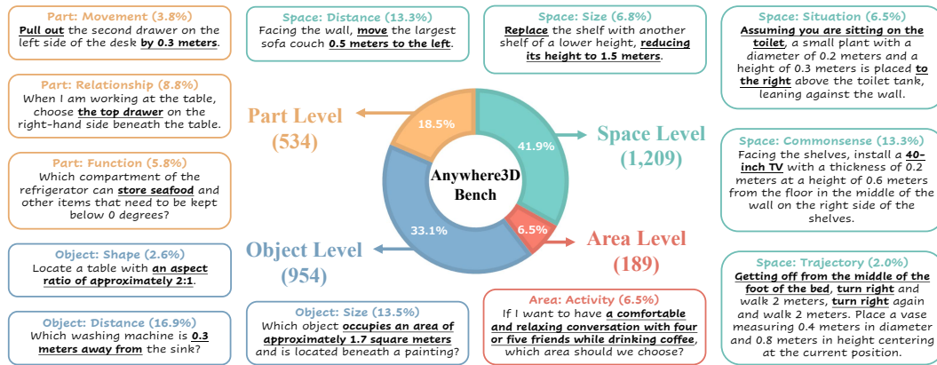
Figure 2: Multi-level visual grounding (Part, Space, Object, Area) with distinct expression types. Emphasized segments highlight phrases aligned with their respective expression type.
