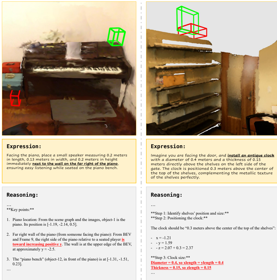
Figure C3: Reasoning process of qualitative examples (a: left) (b: right).
