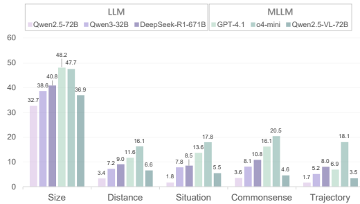
Figure 4: Results on different types of expressions on Space Level.
