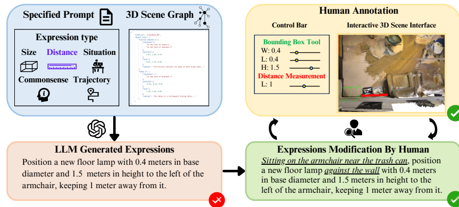
Figure 3: Data generation pipeline of Anywhere3D-Bench. We design specific prompts for different types of expression in four grounding levels. Human annotators are required to annotate the 3D bounding box and refine the GPT-generated expression until they precisely match.
