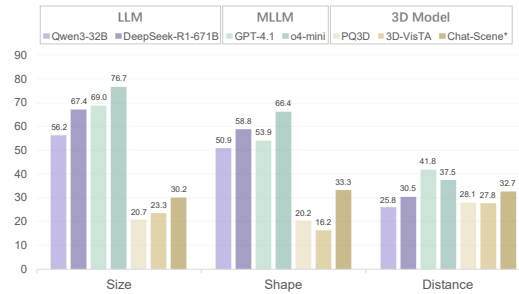
Figure 5: Results on different types of expressions on Object Level.
