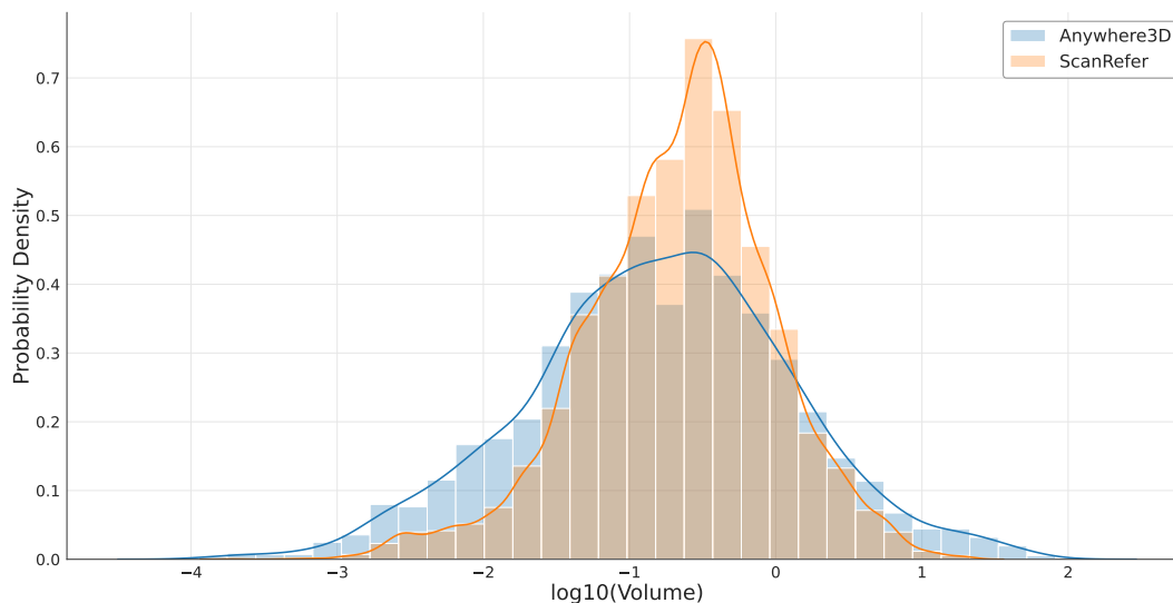
Figure A6: The target objects' volume distribution of Anywhere3D and ScanRefer. Logarithmic scaling is applied to the horizontal axis.
