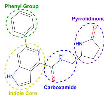
Figure 2: Input molecule
