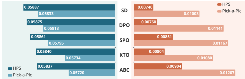
Figure 3: Comparison of Noise Prediction Errors on Pick-a-Pic and HPS. Left: Average noise prediction error \mathbb{E}_{\epsilon,t} [s_{\theta}(\mathbf{x}^+, y)] for the preferred text-image pair (\mathbf{x}^+, y) . Right: Average margin \Delta = \mathbb{E}_{\epsilon,t} [s_{\theta}(\mathbf{x}^-, y)] - \mathbb{E}_{\epsilon,t} [s_{\theta}(\mathbf{x}^+, y)] between the noise prediction errors of the preferred pair (\mathbf{x}^+, y) and the dispreferred pair (\mathbf{x}^-, y) . A lower noise prediction error suggests higher image quality, while a larger \Delta indicates better discrimination aligned with user preference.
