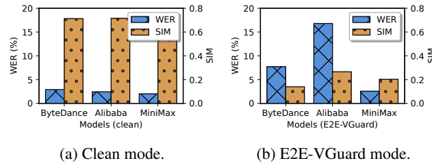
Figure 2: Evaluation of protective performance on commercial APIs.
