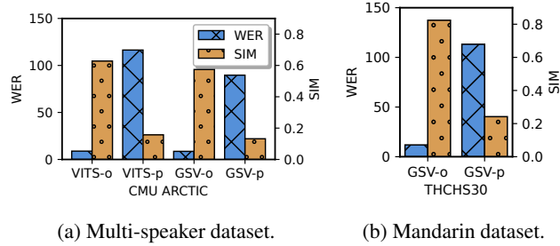
Figure 4: Test results of Multi-speaker and Mandarin datasets.
