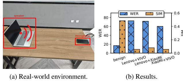
Figure 3: Robust test in the real world. (a) shows the experimental environment. (b) The experimental results. “Lenovo+VIVO” represents the “speaker-microphone”.
