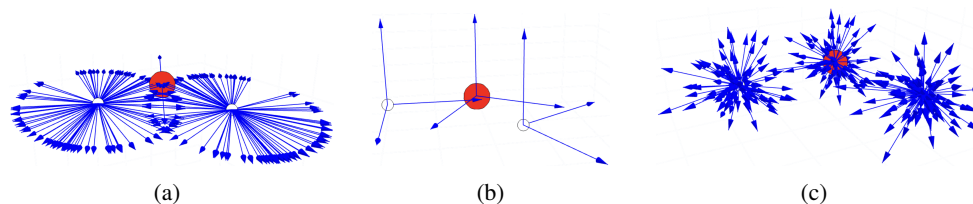
Figure 1: (a) Model output without symmetry-breaking: Equivariant neural networks constrain their output to have the same symmetry as the input. If the input molecule is highly symmetric, this leads to highly constrained Gaussian positions. (b) To solve this issue, ELECTRA initializes each atom's l = 1 vector features with the eigenvectors of the moment of inertia tensor as calculated in that specific atom, which breaks the input symmetry but retains rotational equivariance. (c) Model output after first linear layer with symmetry-breaking: The model can learn its own set of symmetry-breaking vectors, allowing output to not be constrained by the symmetry of the input molecule.
