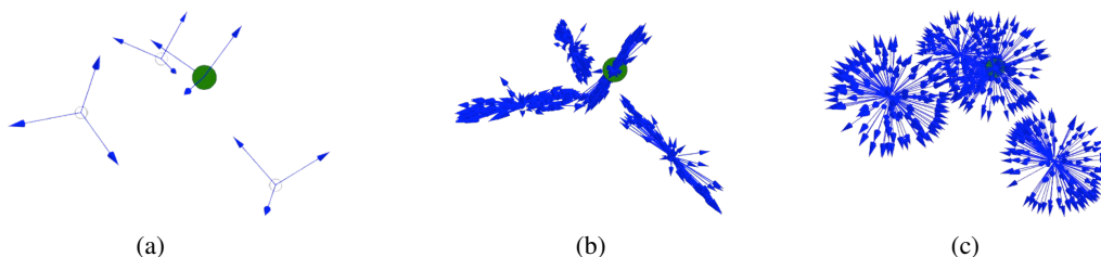
Figure 2: (a) The initial symmetry-breaking objects of the NH 3 molecule (Ammonia). (b) The output of a HotPP model with symmetry-breaking but without debiasing layers: The message passing induces a directional bias that concentrates vectors along certain directions, (c) The output of our model with debiasing layers: The output vectors don't show any visible bias.
