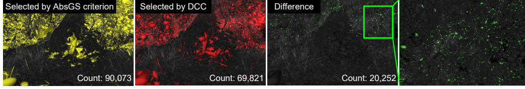
Figure 4: Comparison of split candidates selected by the criterion of AbsGS and DCC from the identical training states. After 14,900 training steps on the Stump scene using the 3DGS, Gaussians selected for splitting are visualized in yellow (AbsGS) and red (DCC). The difference (green) shows (potentially redundant) 20,252 Gaussians are not split by the DCC. Most of these differences are already of tiny sizes, suggesting limited structural gain from further splitting.
