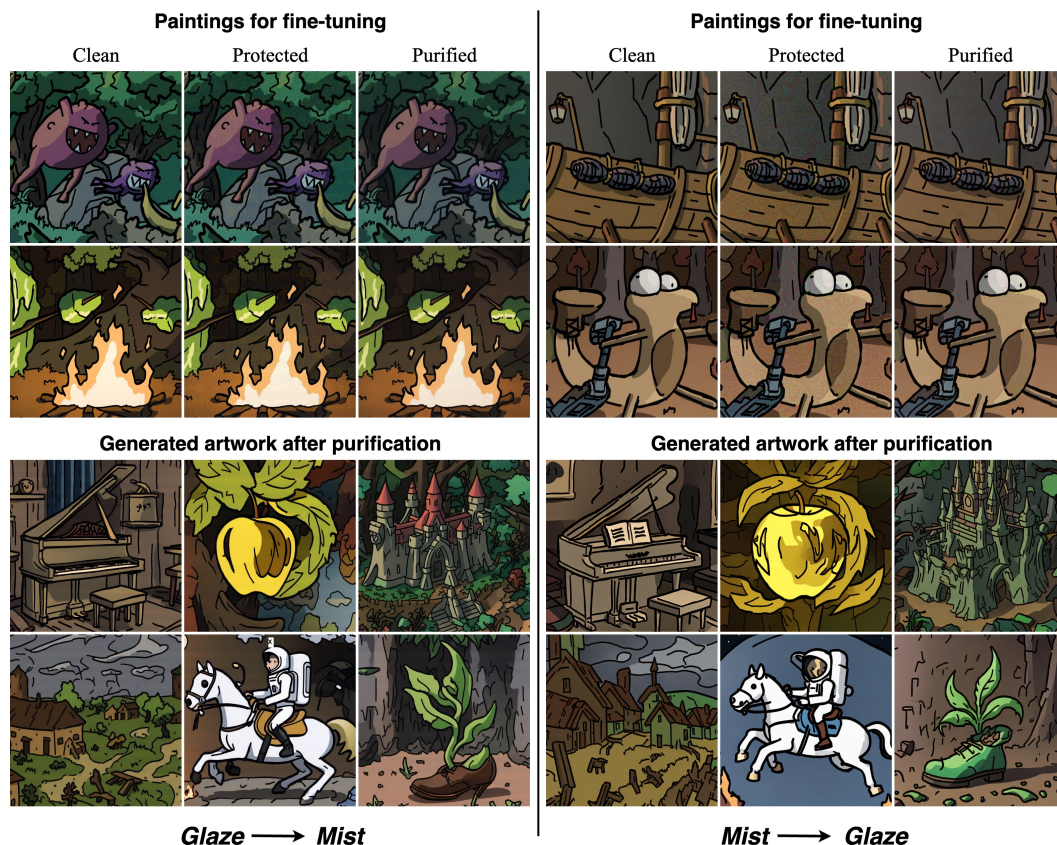
Figure 16: Transferability across style mimicry protections. Left: Using BridgePure-10 trained with (clean, Glaze-protected) pairs to purify Mist-protected paintings. Right: Using BridgePure-10 trained with (clean, Mist-protected) pairs to purify Glaze-protected paintings. Top: Clean paintings by @nulevoy, protected ones, and BridgePure-purified ones. Bottom: Mimicked artwork by prompting the Stable Diffusion v2.1 that is fine-tuned on the BridgePure-purified paintings.
