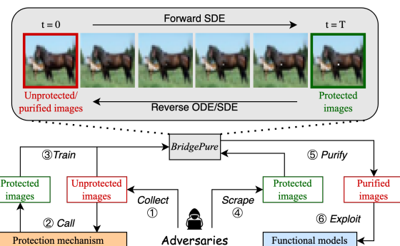
Figure 1: The threat model and illustration of BridgePure. Sequential images show the ODE sampling (purification) process of an example image protected by One-Pixel Shortcut [68].
