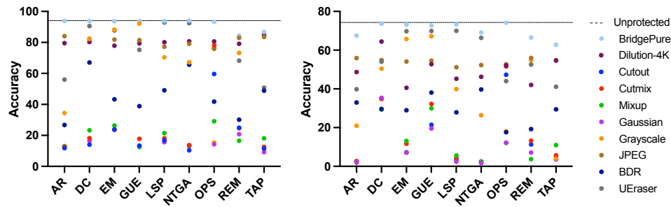
Figure 14: Performance comparison with augmentation-based methods, and protection dilution on CIFAR-10 ( left ) and CIFAR-100 ( right ). The sky blue dots show the performance of BridgePure-0.5. Dots with other colors stand for other circumvent methods. The dashed lines represent the unprotected baselines. The higher the dots, the better the accuracy recovery.
