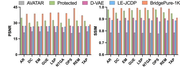
Figure 3: Purification performance against availability attacks that SimCLR evaluates.
