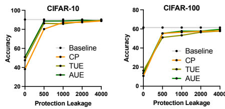
Figure 3: Purification performance against availability attacks that SimCLR evaluates.
