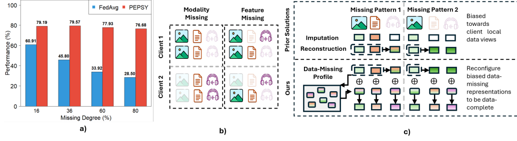
Figure 1: From left to right: (a) Performance comparison showing that FedAvg degrades rapidly with increasing missing data, while our framework PEPSY remains robust; (b) Illustration of two types of data-missing events in MMFL systems: (1) missing modalities and (2) missing input features; (c) Conceptual illustration highlighting the key distinction between our approach and prior work (see Section 2).
