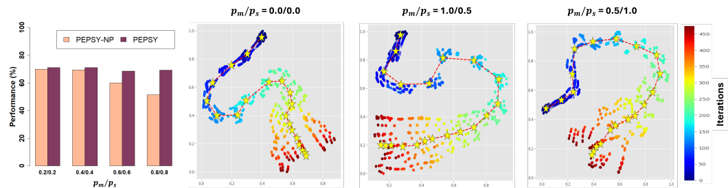
(a) Impact of control pool on proposal's performance under different missing scenarios. (b) Visualization of global control embeddings after 500 training iterations under different missing scenarios. The reduced distance between consecutive iterations indicates convergence, while the variation shows that the embeddings capture different aspects from each client.
