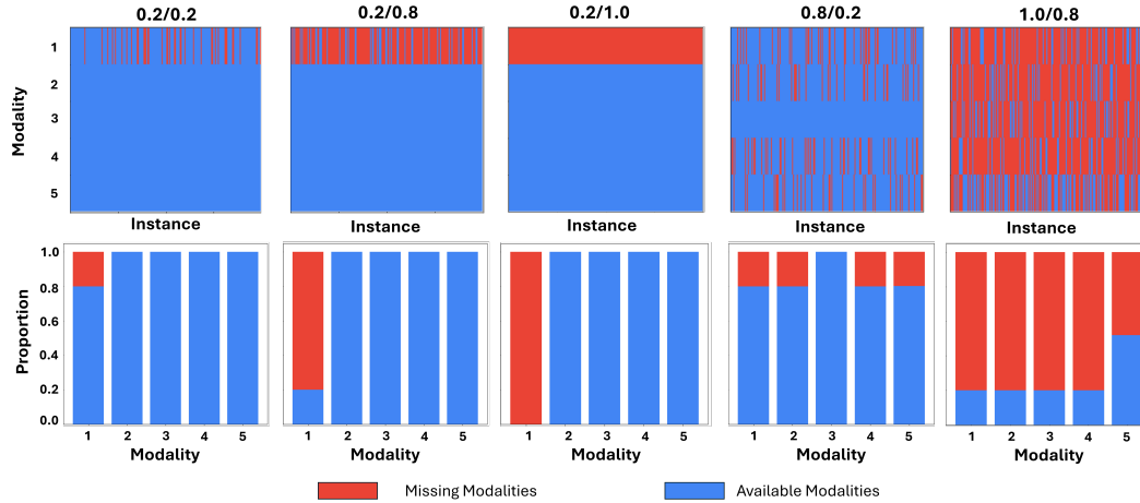
Figure 6: Examples of incomplete datasets \hat{\mathcal{D}} with varying missing statistics ( p_m/p_s ). By controlling these missing statistics, we create diverse evaluation scenarios that reflect real-world conditions.
