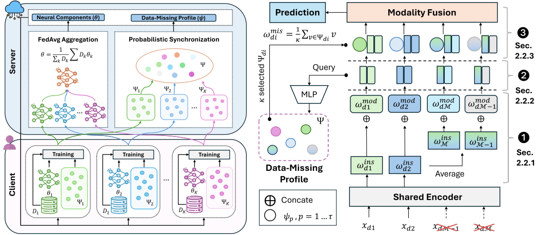
(a) Overall Workflow. PEPsy has two stages: client training and server aggregation. After local training, client parameters are sent to the server to perform aggregation, which includes FedAvg [38] and probabilistic synchronization. (b) Client Design. Each client ① extracts modality- and data-specific features ( w^{ins} , w^{mod} ), then ② queries the data-missing profile \Psi to form w^{mis} as the missing-pattern feature. ③ Finally, w^{mis} reconfigures ( w^{mod} , w^{ins} ) into data-complete features for downstream tasks.
