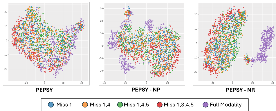
Figure 8: Stability of modality representations under different missing modality scenarios. Ideally, a modality’s representation should remain stable regardless of which other modalities are missing. This stability is not achieved when either the data-missing profile is removed (-NP version) or the reconfiguration signal is omitted (-NR version) from our proposed PEPSY.
