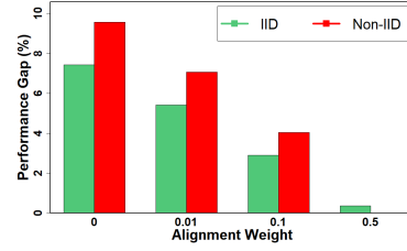
Figure 3: Impact of alignment loss on performance deviation.
