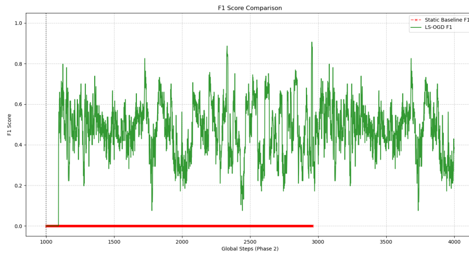
Figure 7: The Comparison between the Static Baseline F1 and LS-OGD F1 over Phase 2
