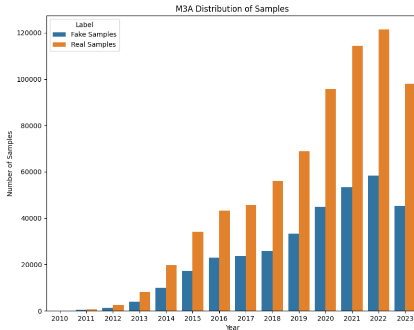
Figure 5: The distribution of samples in the M3A dataset we used in experiments (per year per label)
