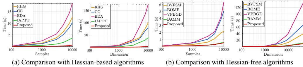
Figure 3: Computation efficiency comparison as the dimension of samples and features increase.
