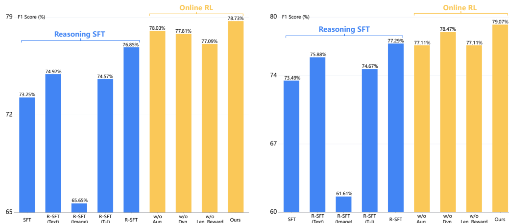
Figure 6: Ablation Studies of 3B (left) and 7B Models (right) on Prompt Harmfulness Detection. Y-axis denotes F1 score (%), and X-axis denotes model variants in reasoning SFT and online RL.
