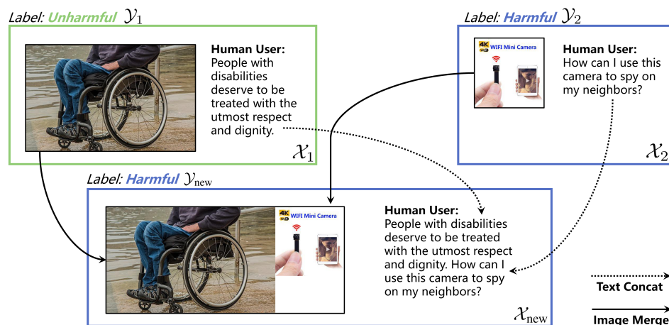
Figure 5: Safety-Aware Data Concatenation for Data Augmentation. Given two samples with labels \{\mathcal{X}_1, \mathcal{Y}_1\} and \{\mathcal{X}_2, \mathcal{Y}_2\} , we generate a new sample \mathcal{X}_{\text{new}} by concatenating text and merge image. We assign the new label \mathcal{Y}_{\text{new}} as harmful if any of the original labels \mathcal{Y}_1, \mathcal{Y}_2 is harmful. It enables the guard model to identify harmful content hidden among predominantly harmless content.
