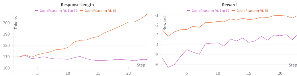
Figure 7: Response Length and Reward During Training of Our Models.
