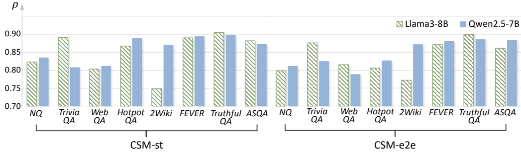
Figure 4: The Spearman correlation ( \rho ) of CSM’s predictions with the oracle CI values.
