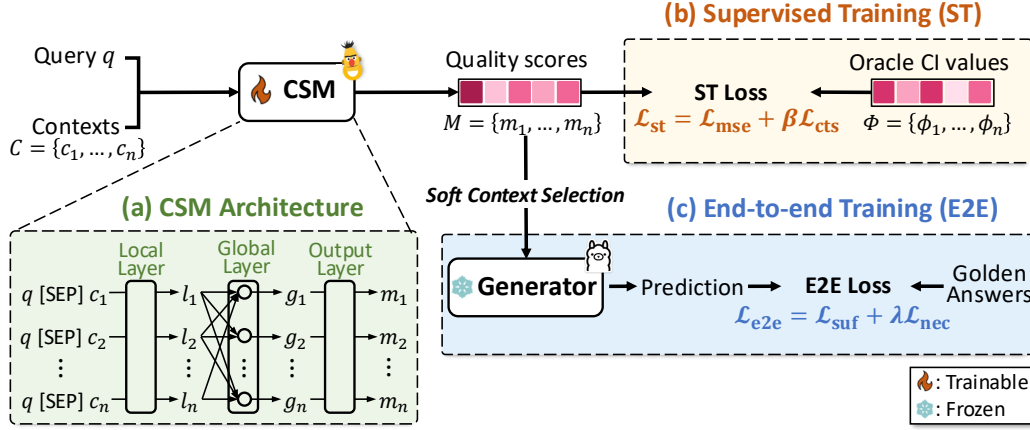
Figure 2: Overview of our proposed CSM: (a) CSM model architecture, (b) supervised training paradigm and (c) end-to-end training paradigm.
