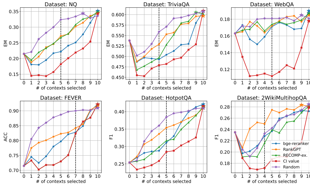
Figure 8: RAG generation performance when selecting poor-quality contexts using different quality metrics, where higher curve indicates better metric. Dashed line marks the top- k cutoff where the average CI value is zero and star marks the top- k yielding best performance. For baselines, we use predicted scores for bge-reranker and RankGPT, and oracle log likelihood scores for RECOMP-ex.
