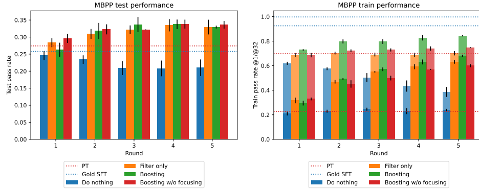
Figure 2: We plot test and train performance of our Algorithm 2 variants on MBPP, across rounds. We report the mean and \text{np.std}(*, \text{ddof}=1) for 3 seeds. For train pass rate plots, we plot both train pass@1 (solid) and train pass@32 (stacked). Boosting results displayed here use weak data (A) .
