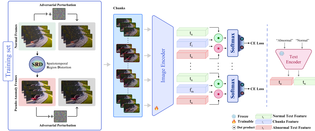
Figure 2: Overview of the FrameShield Framework: (1) The WSVAD training set is constructed using frame-level labels for normal data and frame-level pseudo labels for weakly labeled real anomaly data. Additionally, the Spatiotemporal Region Distortion (SRD) module generates pseudo-anomaly samples with precise frame-level annotations, further augmenting the training set with adversarial perturbations. (2) Two predefined prompts, "normal" and "anomaly," are used to extract text embeddings from the frozen text encoder. (3) Training videos are segmented into chunks and processed by the XClip-based encoder. The dot product between each chunk's feature representation and the text prompt embeddings is computed to obtain normality and abnormality scores, optimizing the network through chunk-level cross-entropy loss.
