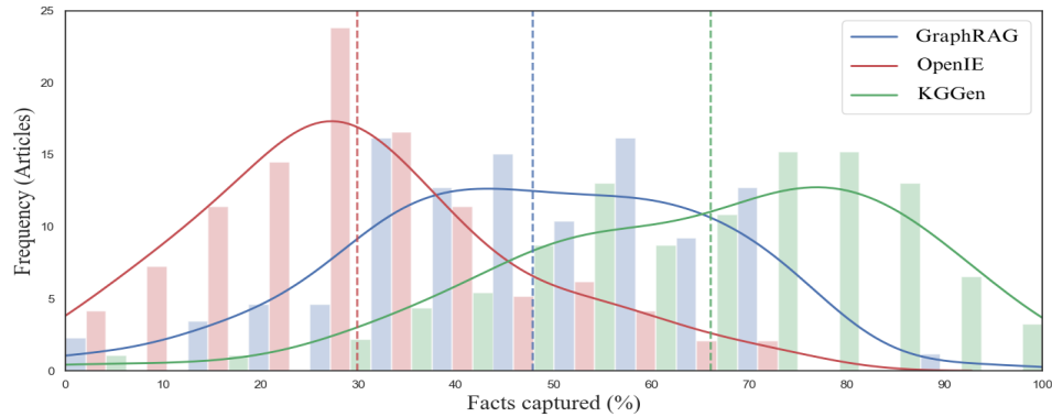
Figure 3: Distribution of MINE-1 scores across 100 articles for GraphRAG, OpenIE, and KGGen. Dotted vertical lines show average performance. KGGen scored 66.07% on average, significantly outperforming GraphRag 47.80% and OpenIE 29.84%.
