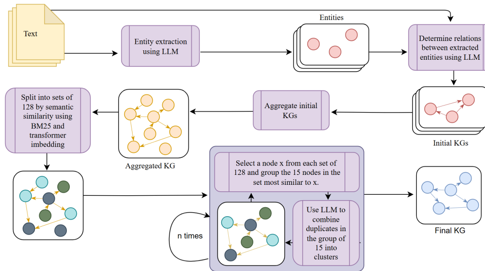
Figure 1: KGen extraction method
