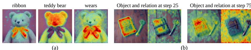
Figure 2: (a) Attention maps [15] for various semantic primitives. Caption: A teddy bear wearing a red ribbon around its neck. Attentions exhibit significant overlap between the object primitive ‘ribbon’ and relation primitive ‘wears’, resulting in semantic entanglement. (b) Superimposed attention maps of object primitive type and relation primitive type at denoising timesteps 25 and 75, respectively. Notably, the model focuses more on object primitives during the earlier stage and shifts more attention to relation primitives in the later stage.
