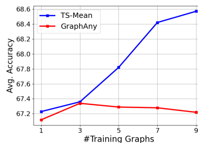
Figure 3: Average zero-shot accuracy of TS-Mean and GraphAny across 20 datasets as a function of the number of training graphs.
