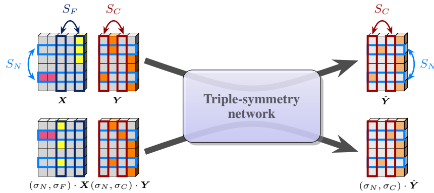
Figure 1: The input to a triple-symmetry network is a feature matrix X and (possibly masked) label matrix Y . The encoder must be equivariant to element-wise permutations \sigma_N \in S_N (affecting the rows of both X and Y ), equivariant to class label permutations \sigma_C \in S_C (affecting the columns of Y ), and invariant to feature permutations \sigma_F \in S_F (affecting the columns of X ).
