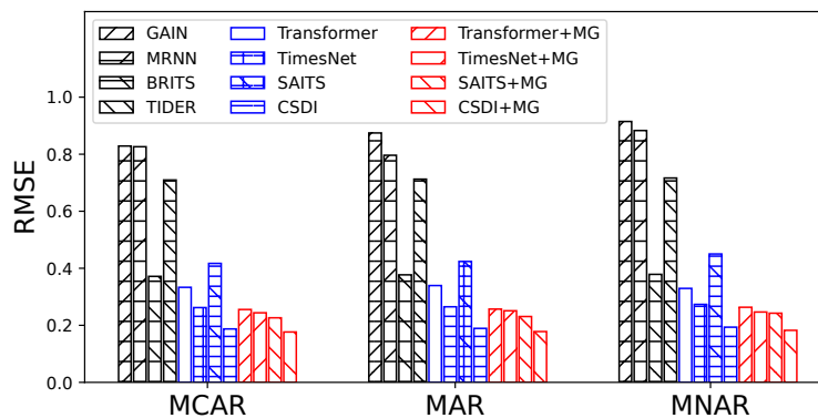
Figure 7: Varying the missing mechanism over ETTh1 dataset with 10% missing values.
