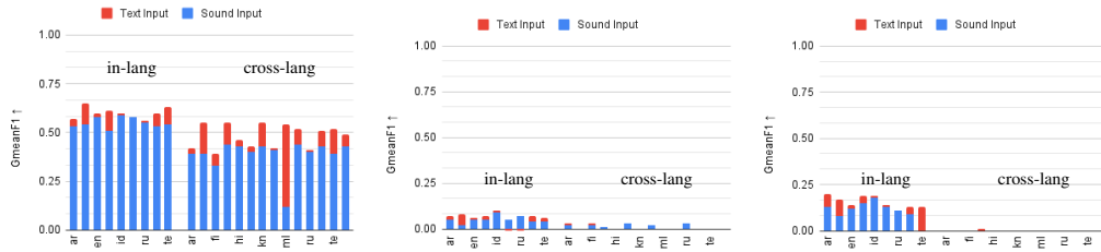
Figure 9: MSEB span reasoning tasks: Generative (Gemini) vs retrieval (Gemini embedding and Gecko) approach.
