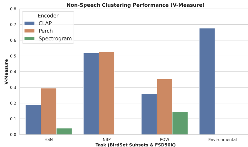
Figure 17: Clustering performance on non-speech domains. Perch excels in its specialized domain of bioacoustics (BirdSet), while CLAP demonstrates strong generalist capabilities across both environmental and bioacoustic tasks.
